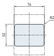
[Drilling holes for mounting]
