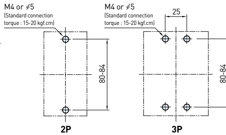
[Panel cut-out]
