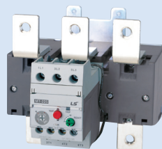
MT-225 Overload relay directly mountable to the contactor Current range 65-240A ► 93 page
